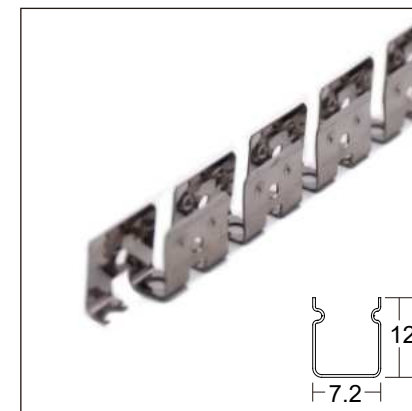
Molded clip, stainless steel clip, 100m/carton
