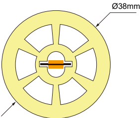
Part No.:YT-C38 PCB Width:10mm LED strip light: LT-2835WW120R-W24
