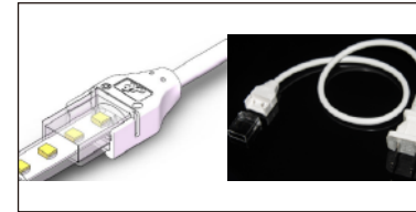
2PIN- 10MM IP65 AC220V With cable and plug PCB to cable
