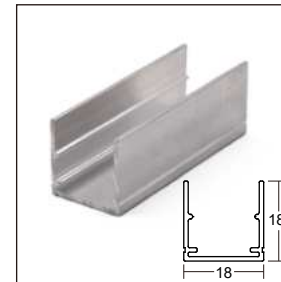
Aluminous clip, 18x18mm Mini. Size:5cm
