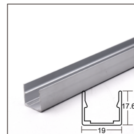
Aluminous clip, 19x17.6mm
