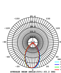
LUMINOUS INTENSITY DISTRIBUTION
