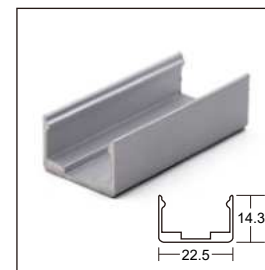
Aluminous clip, 22.5x14.3mm Mini. Size:5cm
