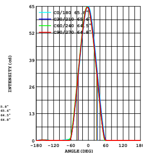
LUMINOUS INTENSITY DISTRIBUTION
