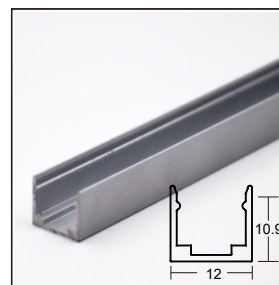
Aluminous clip, 12x10.9mm
