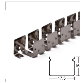
Molded clip, stainless steel clip, 100m/carton
