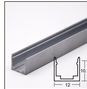
Aluminum clip, 12x10.9mm
