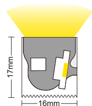
Section Dimension
