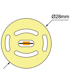
Part No.:YT-C28 PCB Width:8mm LED strip light: LT-2835WW120R-W24
