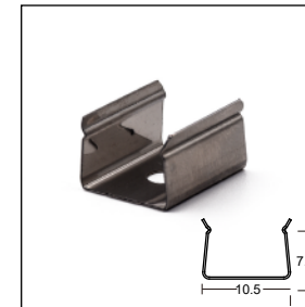
stainless steel clip
