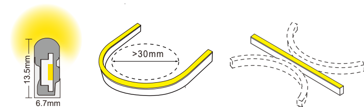
Section Dimension
