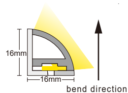
Section Dimension
