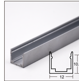
Aluminous clip, 12x10.9mm
