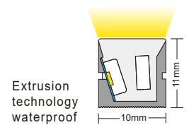
Section Dimension
