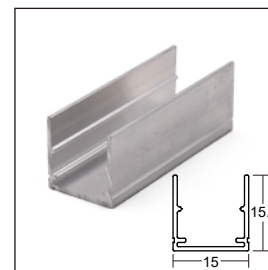
Aluminous clip, 15x15.6mm
