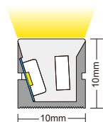
Section Dimension
