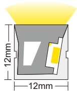
Section Dimension
