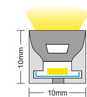
Section Dimension
