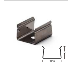
stainless steel clip
